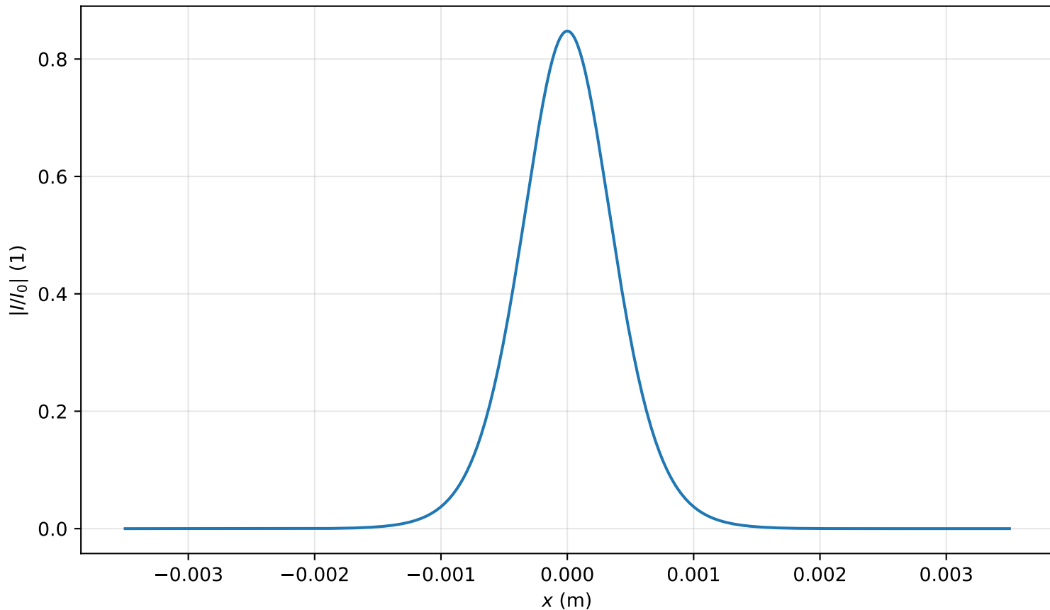
Intensity profile I(x, y = 0, z = 1.911m)/I_0 , P_{in}=0.5P_{cr} , artificial time
